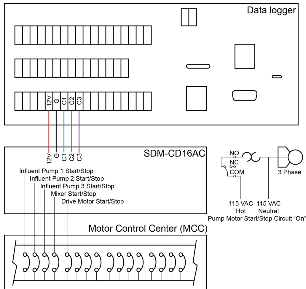
FIGURE 4-3. SDM-CD16AC relay outputs to MCC
